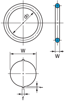
O-Ring Dimensions
