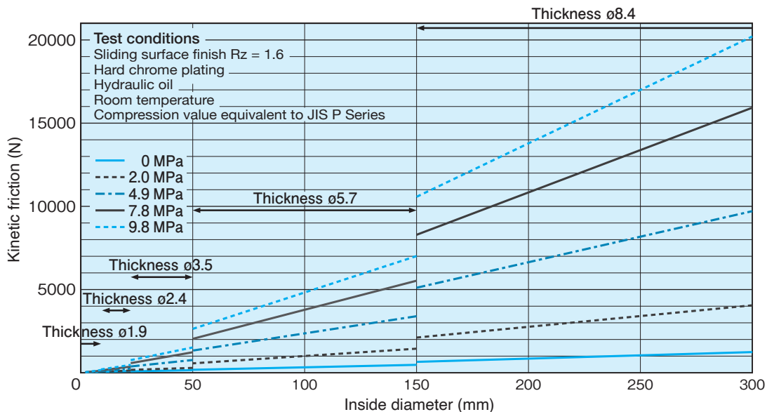
Fig. 6-4 O-Ring Kinetic Friction
