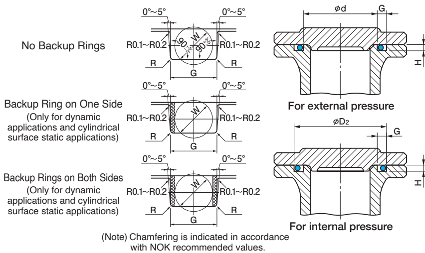
Groove Shapes For Flat Face Static Applications
