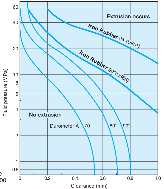
Fig. 1-3 O-Ring Extrusion Limits
